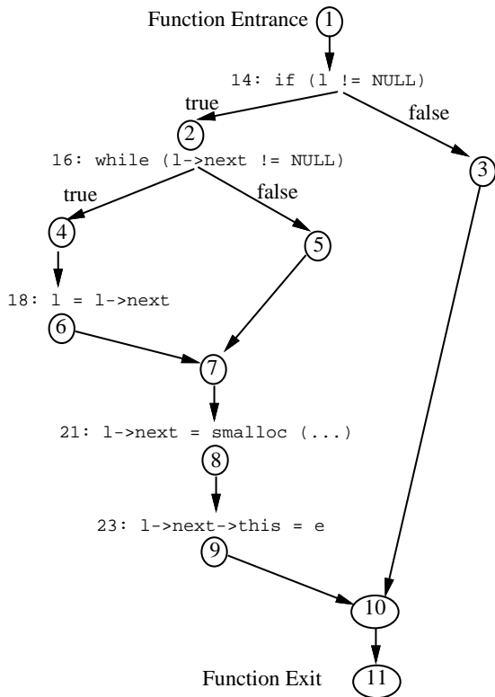
Figure 6: Control flow graph for list_addh .
